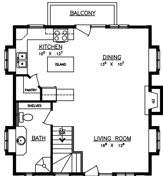
SECOND FLOOR AREA = 624 S.F.
