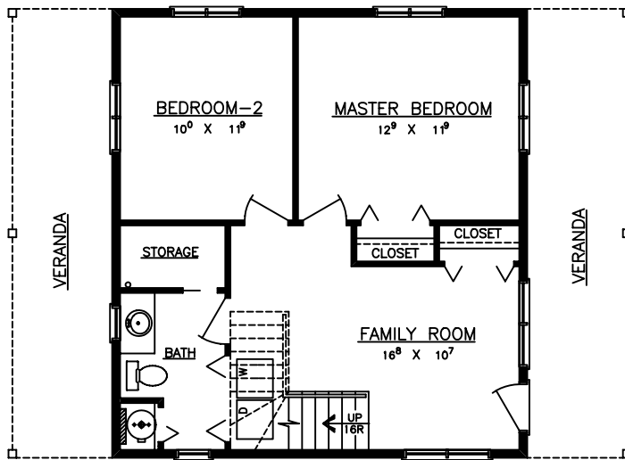
MAIN FLOOR AREA = 624 S.F.
